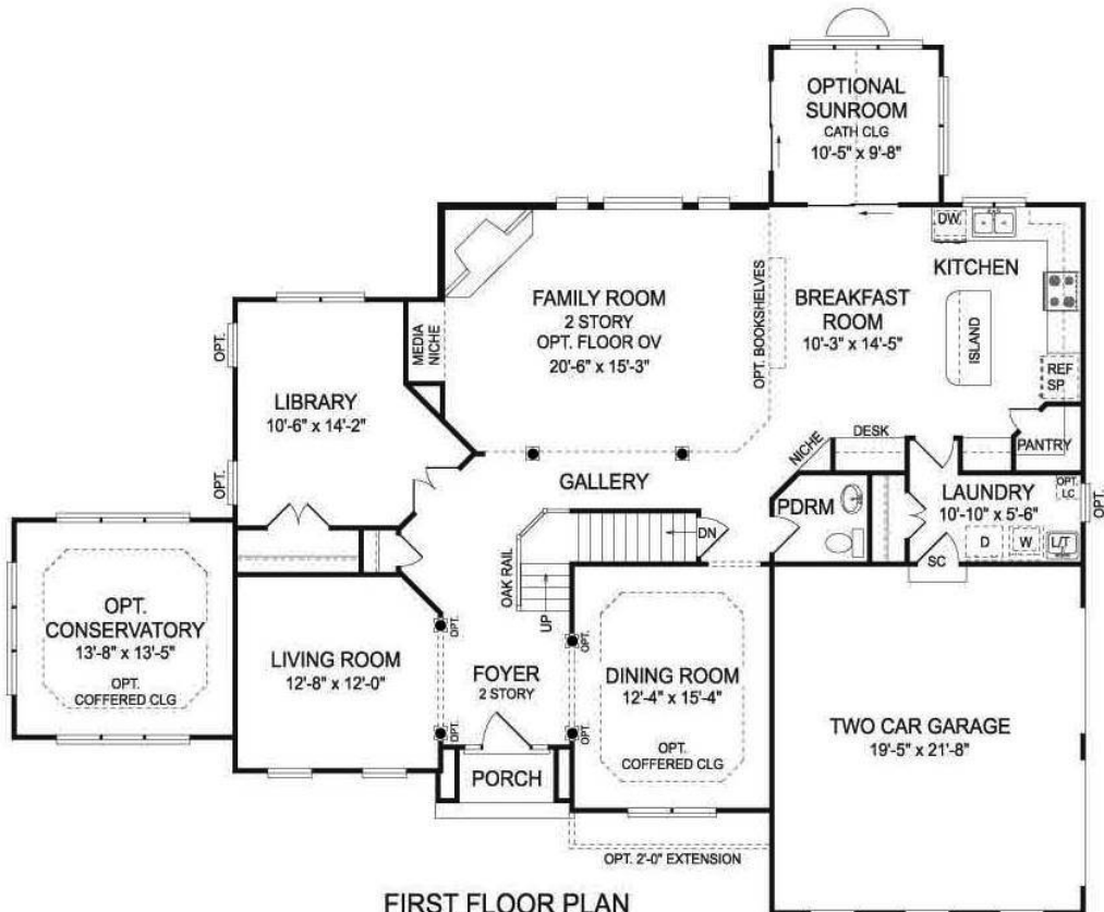
FIRST FLOOR PLAN THE YORKSHIRE MANOR
